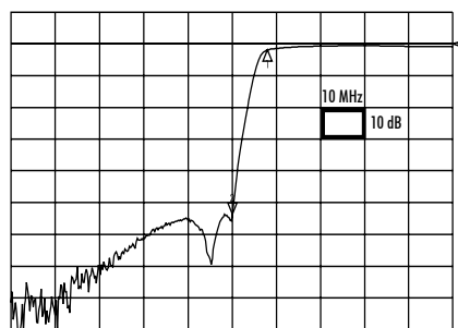
Typical Frequency Response of 5KHP
